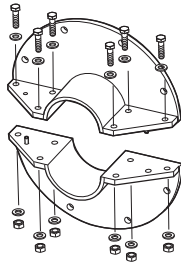
SLFO sleeve
