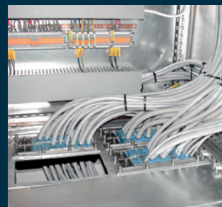
Gabinetes DCS/PLC
